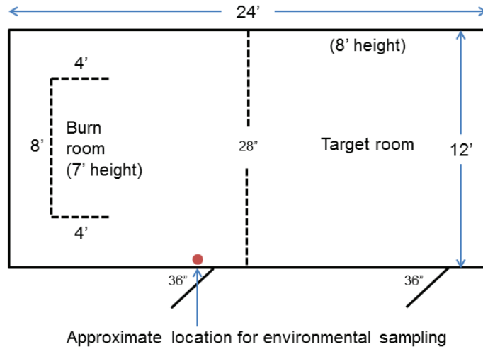
Figure 1. Schematic showing the interior layout of the burn structure used in round 1.
