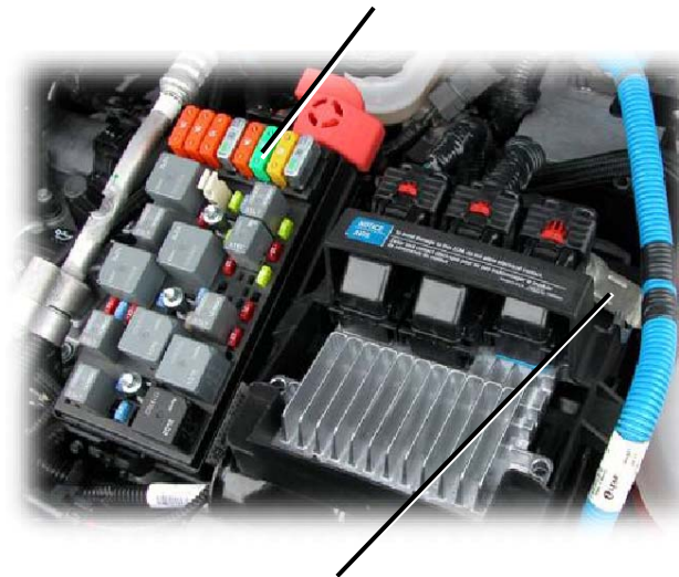
30 amp Ignition Maxi Fuse
